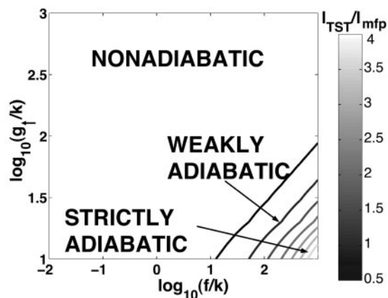
Fig. 3. A phase diagram as a function of the activated production rate g_{\uparrow} and the unbinding rate f for constant K^{eq}V^2 , showing the areas of parameter space where a given escape mechanism dominates based on the ratio of the size of the transition-state region l_{TST} to the mean free path l_{mfp} . If the number of crossings of the separatrix is large, l_{TST}/l_{mfp} > 1 , the transition is adiabatic. If the system commits to a new attractor after one crossing, l_{TST}/l_{mfp} < 1 , the transition is nonadiabatic.
