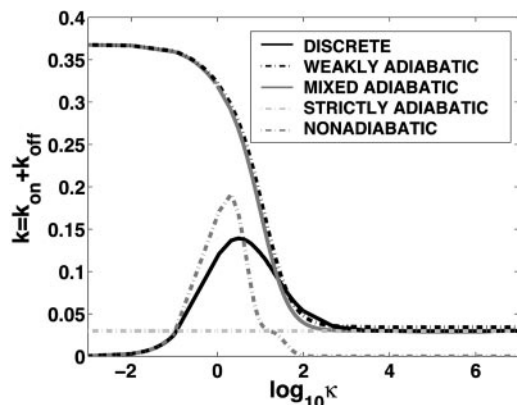
Fig. 1. The sum of the escape rates k = k_{\text{on}} + k_{\text{off}} as a function of the adiabaticity parameter \kappa = (hg_{\uparrow}^2)/(2k^3) for a self-activating switch with g_{\uparrow} = 100 , g_{\downarrow} = 8 , k = 1 , n_N^{\uparrow} = 53.4 . Comparison of the exact discrete n numerical calculation based on the mean free passage time (black solid line), with approximate methods: in the nonadiabatic limit (small \kappa ) (gray dashed line; Eqs. 1 and 3), in the weakly adiabatic regime (black dashed line; Eqs. 5 and 8), and mixed crossover regime (gray solid line). The adiabatic results tend asymptotically to the strictly adiabatic limit (large \kappa -flat escape rate) (light gray dashed line; Eqs. 6 and 9). In the strictly adiabatic limit the binding of transcription factors to the DNA-binding site is equilibrated. In the nonadiabatic and weakly adiabatic limits the escape rates show a dependence on the adiabaticity parameter; the process is influenced by the DNA-binding state fluctuations.
