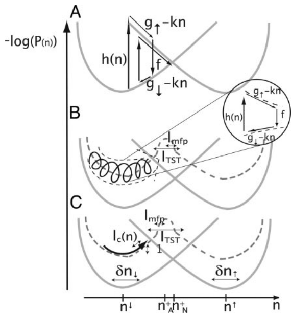
Fig. 2. A schematic diagram of the difference in the character of the transitions from the state with a small mean number of proteins to the state with a large mean steady-state number of proteins in the nonadiabatic (A) where the escape rate is given by Eqs. 1 and 3, adiabatic (B) where the escape rate is given by Eqs. 5 and 8, and extremely adiabatic (C) regimes. The dark gray dashed line marks the effective potential for protein number change. The horizontal arrows signify binding and unbinding events.
